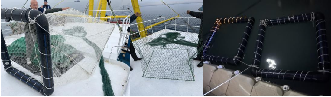
Figure 14. Experimental cages used for long-term survival trials (Left: Cage constructed with knotless polyamide (PA) netting (20 mm mesh). Middle: Cage constructed with knotted polypropylene (PP) netting (150 mm mesh). Right: Cages deployed at sea during the experiment.)
