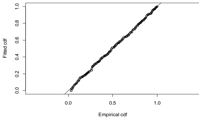
Q-q plot
