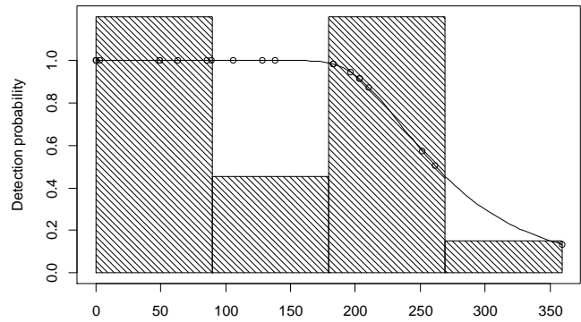
Detection function
