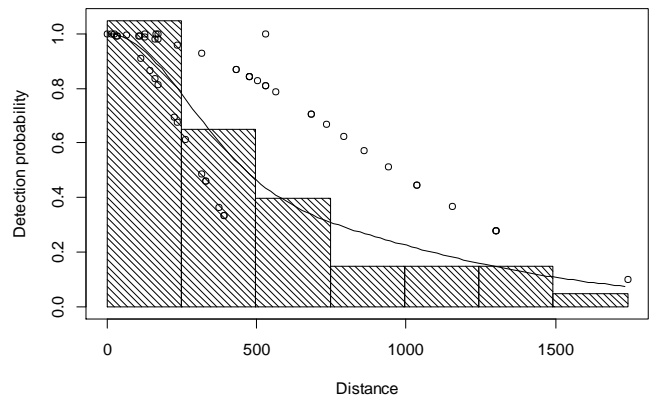
Detection function
