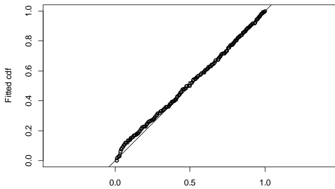
Q-q plot
