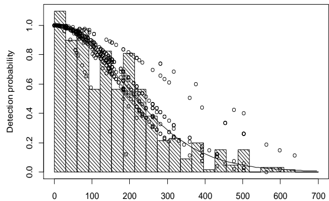
Detection function
