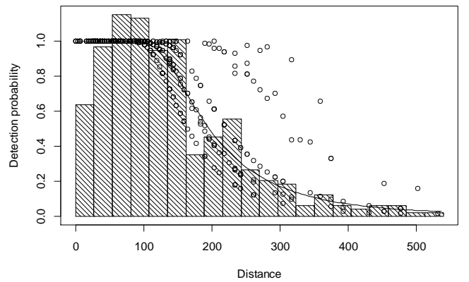
Detection function
