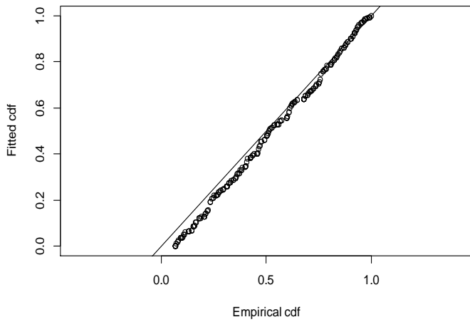
Q-q plot
