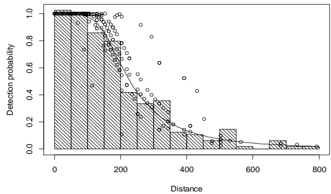
Detection function
