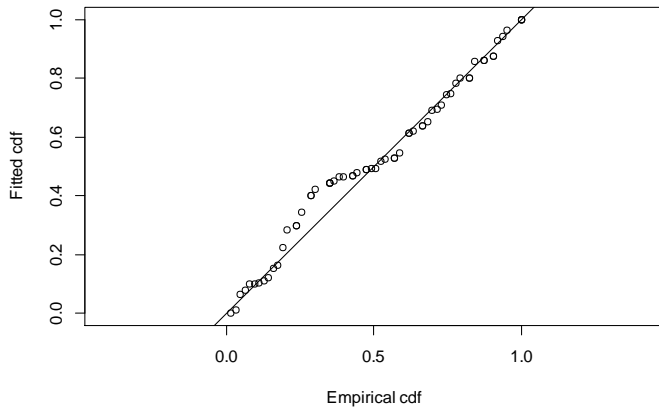
Q-q plot
