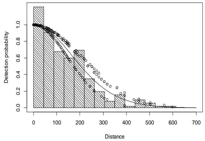
Detection function
