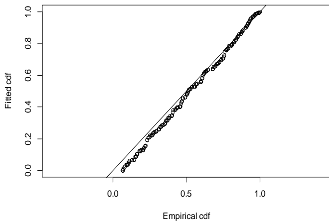
Q-q plot
