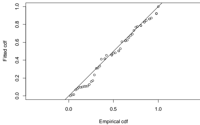
Q-q plot
