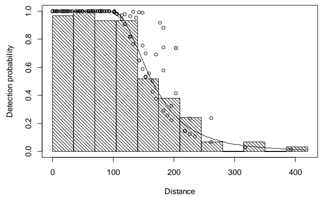
Detection function
