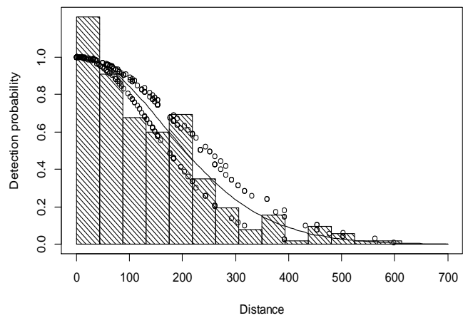
Detection function
